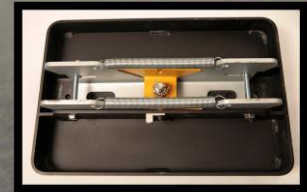
Bottom View of Lid in Unlocked Position – Pick Holes Unblocked
