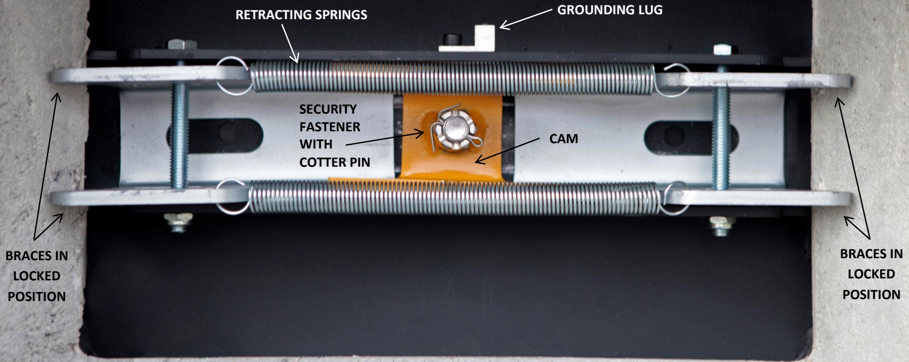
K-Series LockLid™ Inserted Into a Christy N-09 Pull Box and in Locked Position
